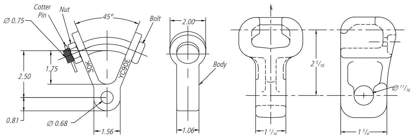
Socket Eye "SE" Suffix
