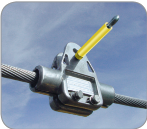
5. Remove the "Hot Stick" from the Live-line Attachment Tool
