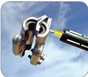
2. Secure the HIBUS Suspension to the "Hot Stick" using the Live-line Attachment Tool
