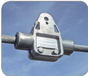
8. Remove the Live-line Attachment Tool with the "Hot Stick" and attach the HIBUS Suspension to the insulator with the mounting pin provided
