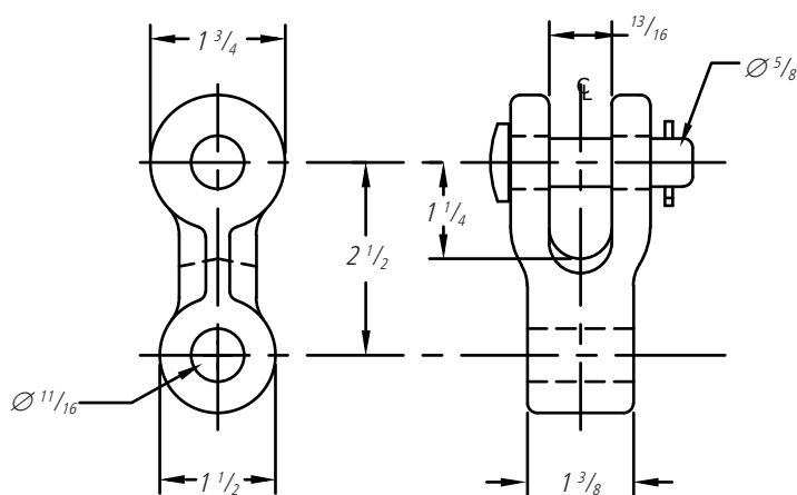
Clevis Eye "SCE" Suffix
